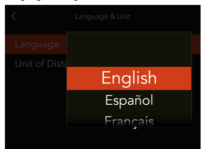
Language Setting
