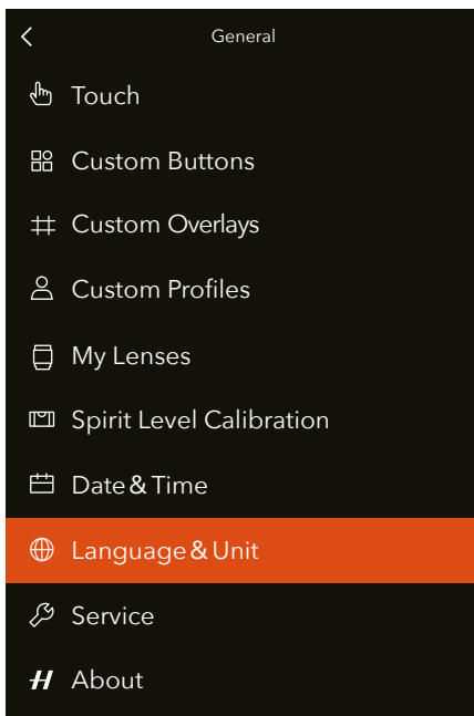
Language Menu
